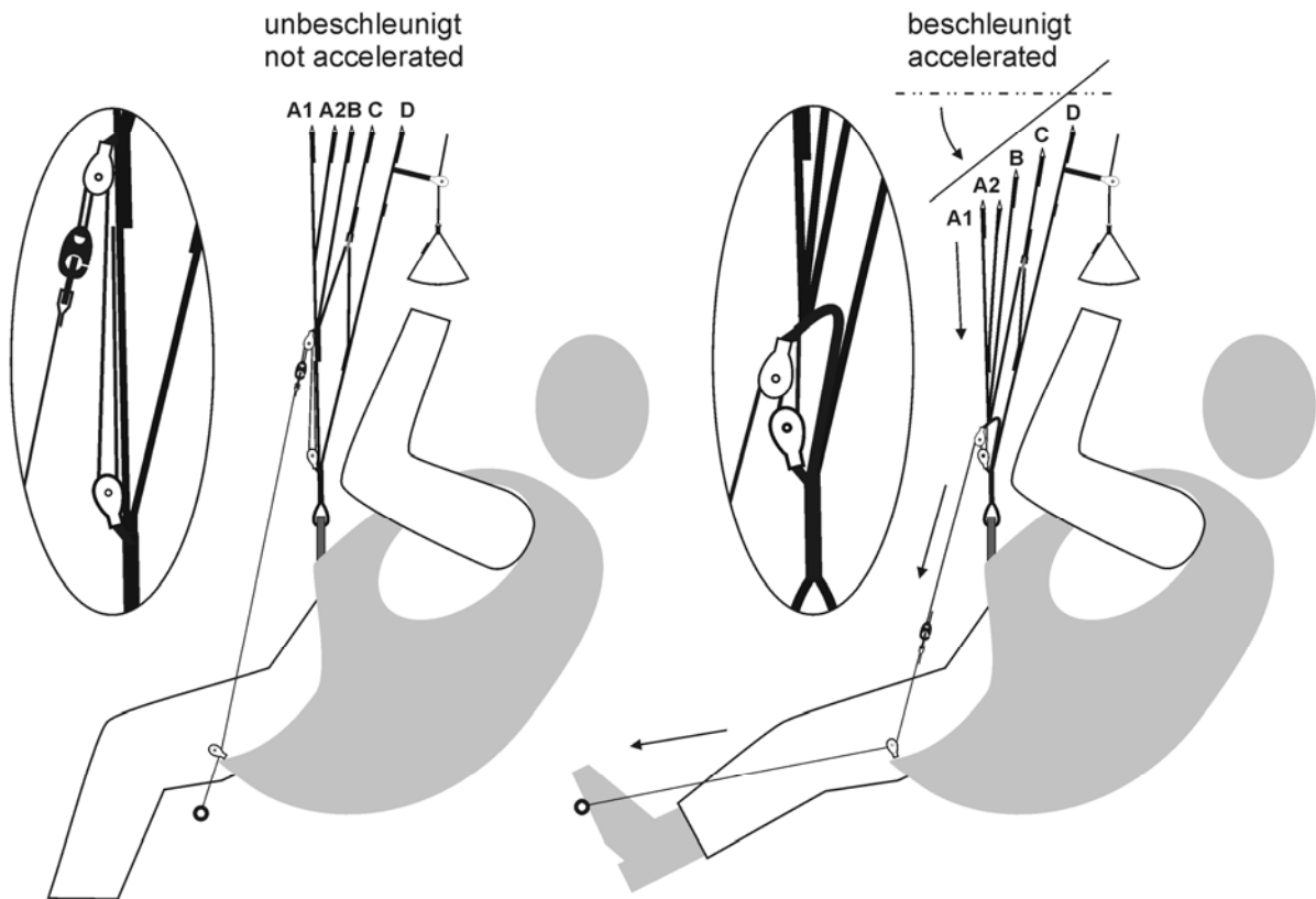
Figure 2: How the Speed system of the ARCUS 6 works
