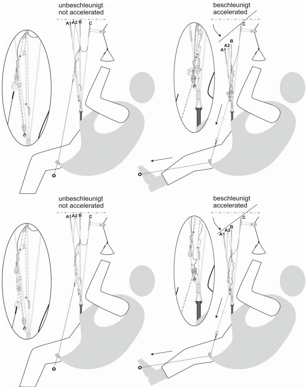
Fig. 8 How the MIURA RS speed system works (MIURA RS without speed limiter top figure, MIURA RS with speed limiter bottom figure)
