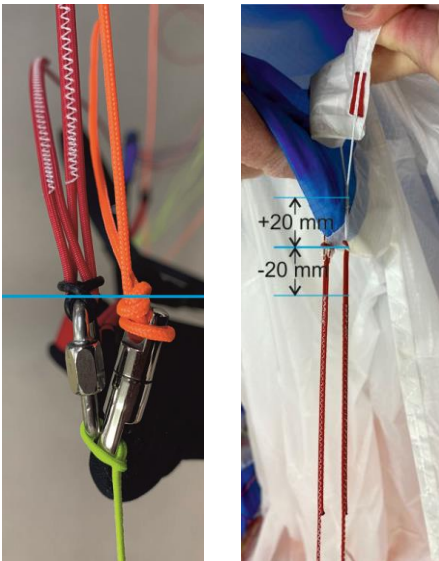
Fig. 14 Measuring points for the quick brake line check
