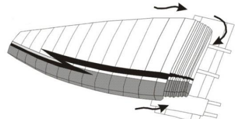
Fig. 6c: Now place the protection bag underneath the section of the glider which has been folded together, and turn it around 90°, so that the ribs are all lying along the length of the protection bag. Then continue as in the second step, placing the leading edges one on top of the next until you reach the tip of the glider.
