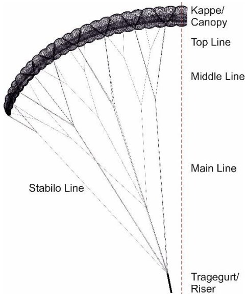
Fig. 1: CAD drawing of Astral 7
