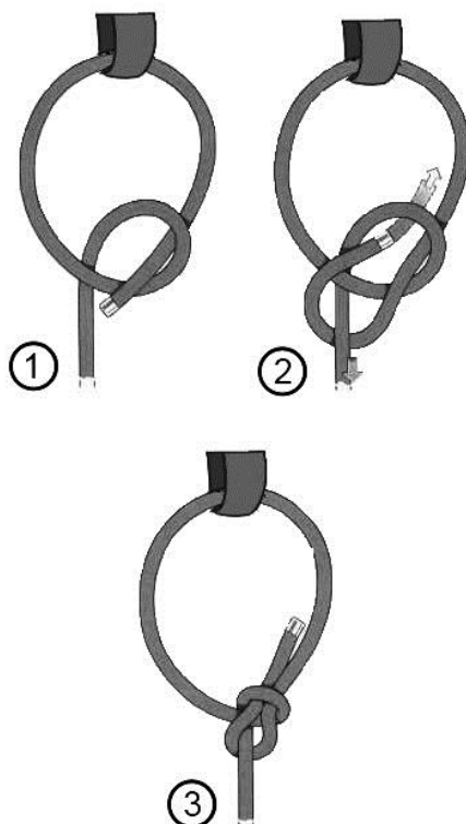
Fig. 3: Bowline knot
