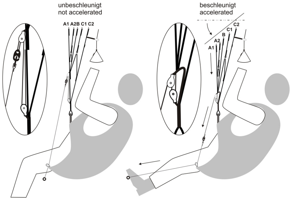
Fig. 5: How the Stratus 8 speed system works
