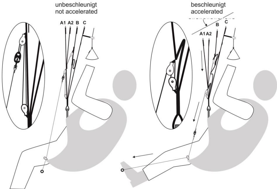
Fig. 7 How the APUS RS speed system works
