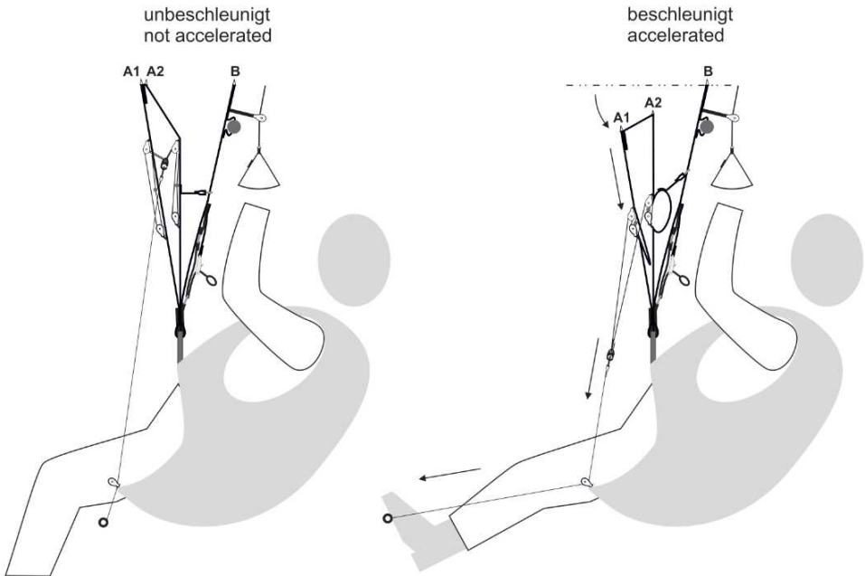
Fig. 5: How the Core 2 speed system works
