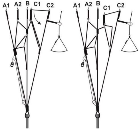
Fig. 9 Adjustment of flightdirection by C-bridge
