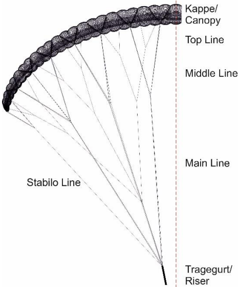
Fig. 1 CAD drawing of NYOS RS
