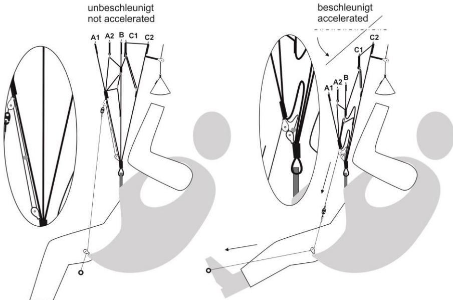
Fig. 7 How the NYOS RS speed system works
