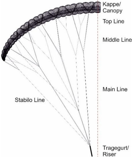
Fig. 1 CAD drawing of VERSO RS
