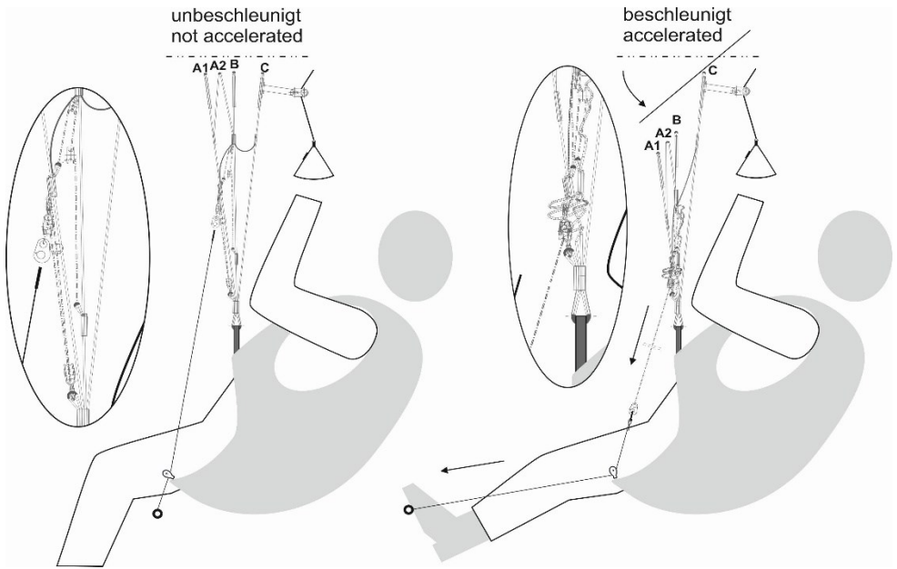
Fig. 6 How the VERSO RS speed system works
